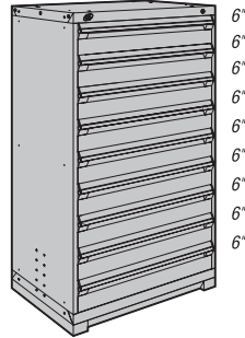
9 drawers R5AEC-5813 36" x 18" x 60" R5AEE-5813 36" x 24" x 60"
