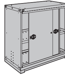
1 sliding door / 1 adjustable shelf / 1 bottom shelf R5AHE-4416 48" x 24" x 46" R5AHG-4416 48" x 27" x 46"
