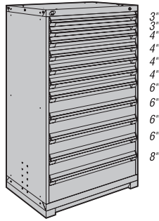
11 drawers R5AEC-5803 36" x 18" x 60" R5AEE-5803 36" x 24" x 60"
