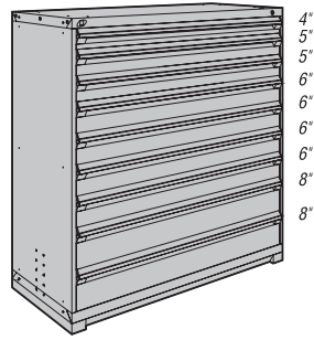
9 drawers R5AKE-5803 60" x 24" x 60" R5AKG-5803 60" x 27" x 60"
