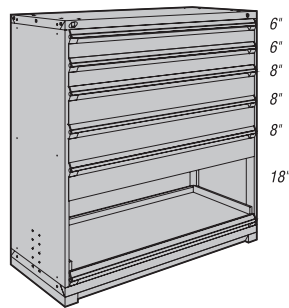
5 drawers / 1 roll-out shelf R5AKE-5801 60" x 24" x 60" R5AKG-5801 60" x 27" x 60"
